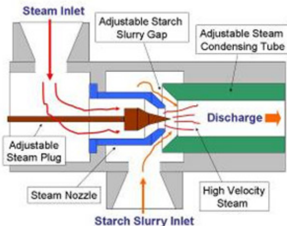
PSX Jet cooker Internal View
