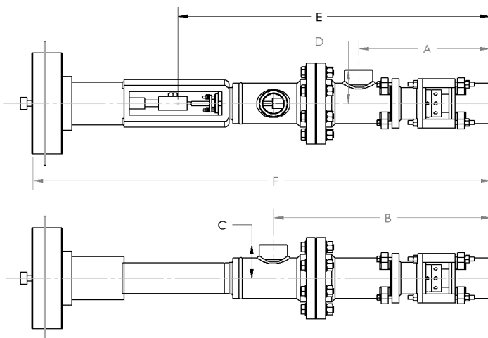
PSX Jet Cooker – Dimensions & Weights
